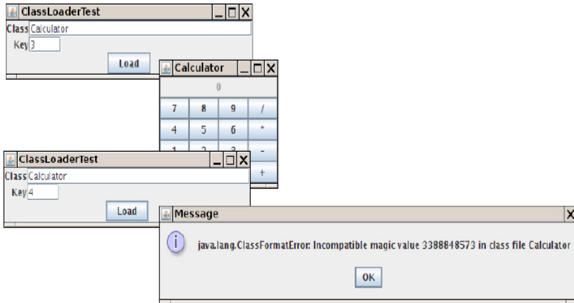
Figure 10.3 The ClassLoaderTest program
