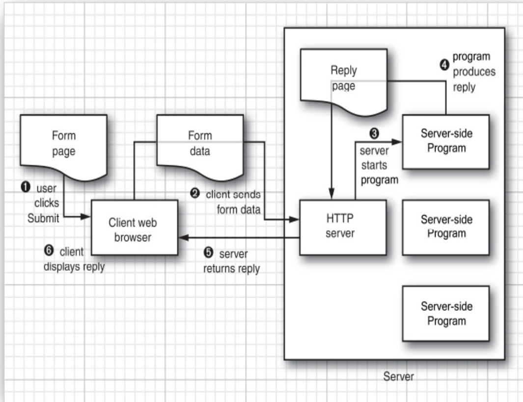
Figure 4.8 Data flow during execution of a server-side program
