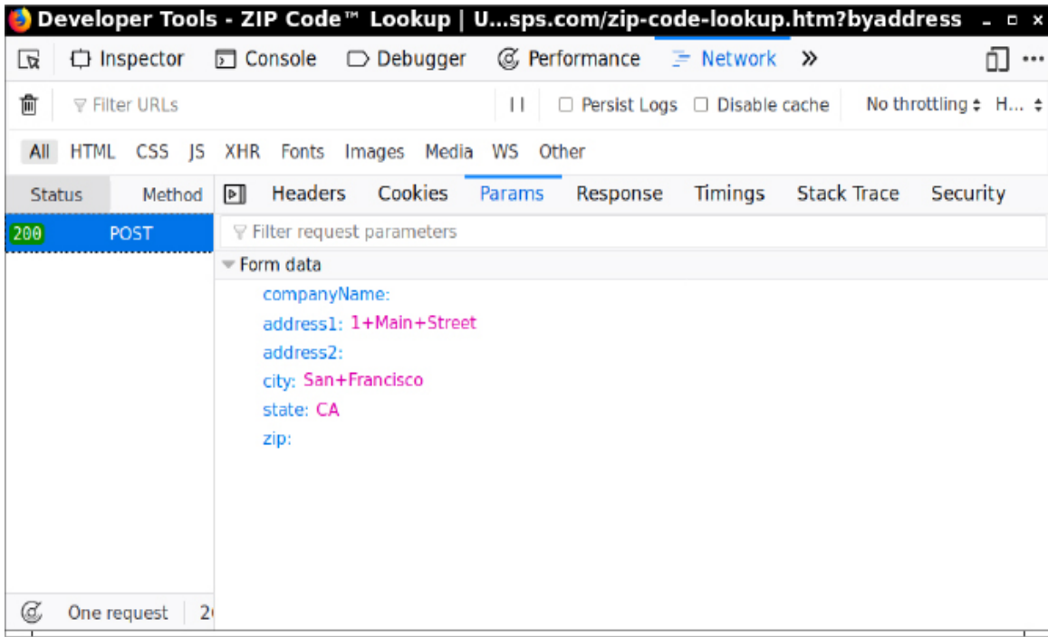
Figure 4.9 Monitoring the submission of a form
