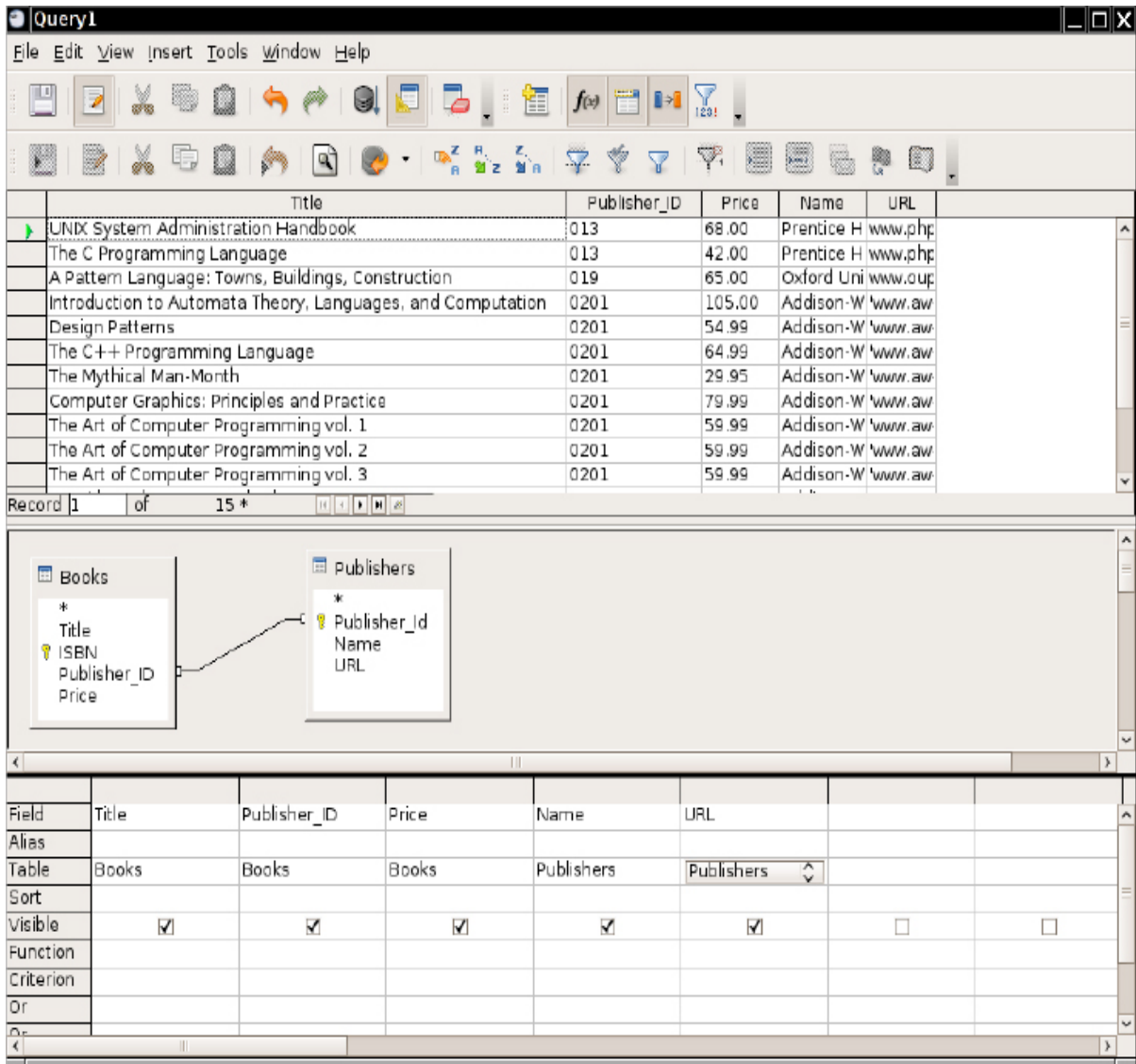
Figure 5.4 Two tables joined together
