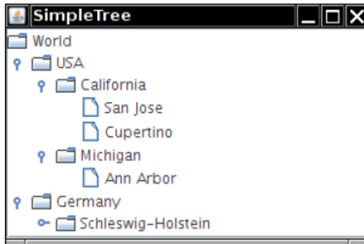
Figure 11.18 A tree with no connecting lines
