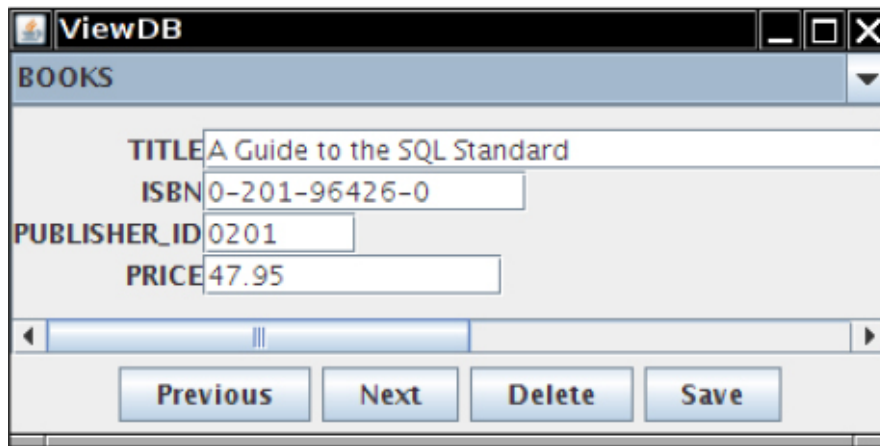
Figure 5.6 The ViewDB application
