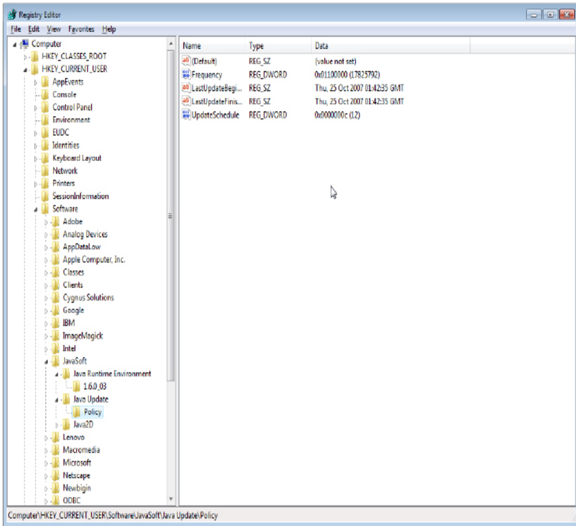
Figure 12.4 The registry editor
