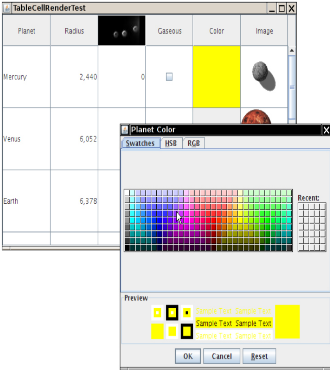
Figure 11.10 Editing the cell color with a color chooser
