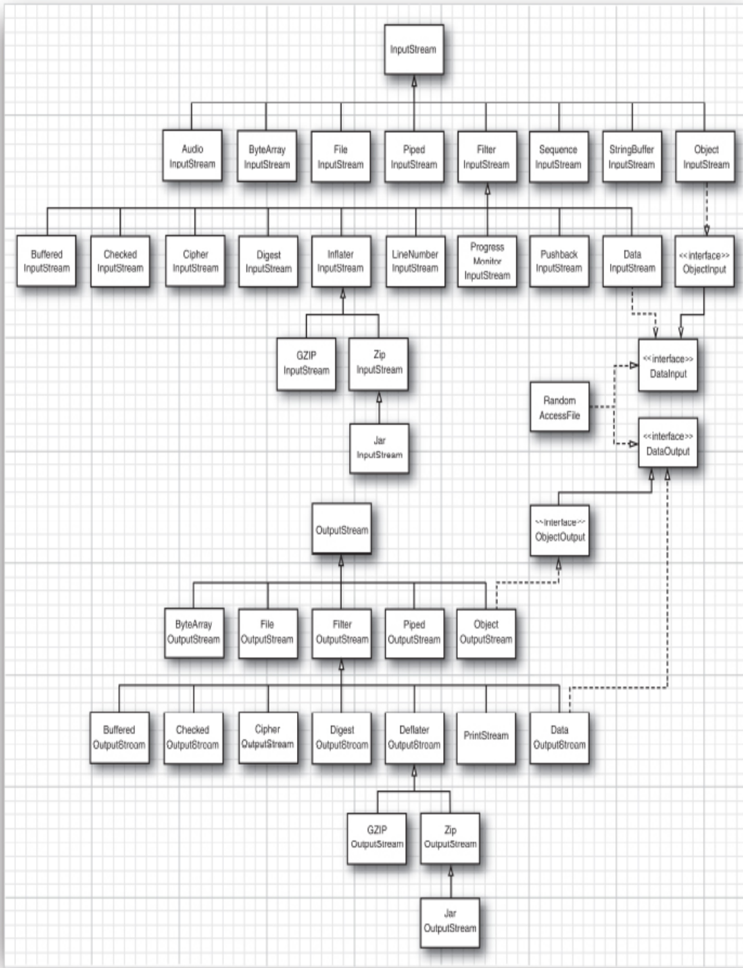
Figure 2.1 Input and output stream hierarchy
