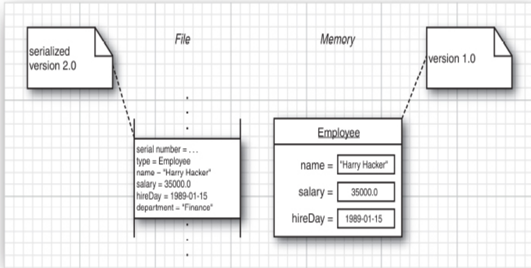
Figure 2.7 Reading an object with fewer instance fields
