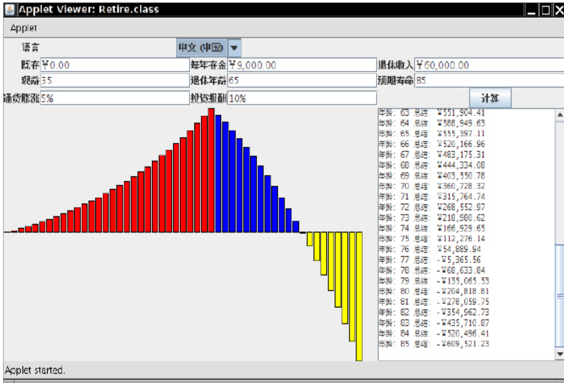
Figure 7.6 The retirement calculator in Chinese
